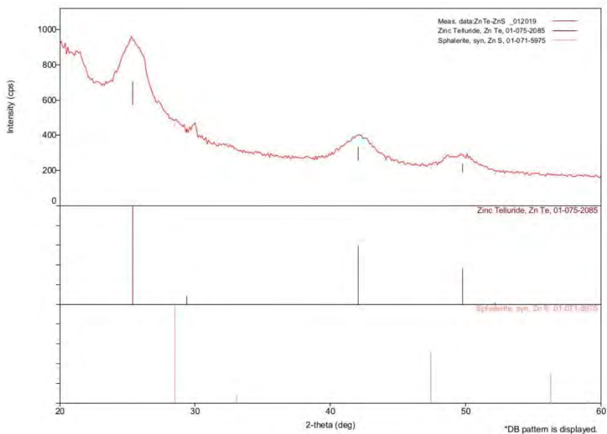
Figure 22: Intensity of X-ray diffraction from ZnTe/ZnS QDs.
