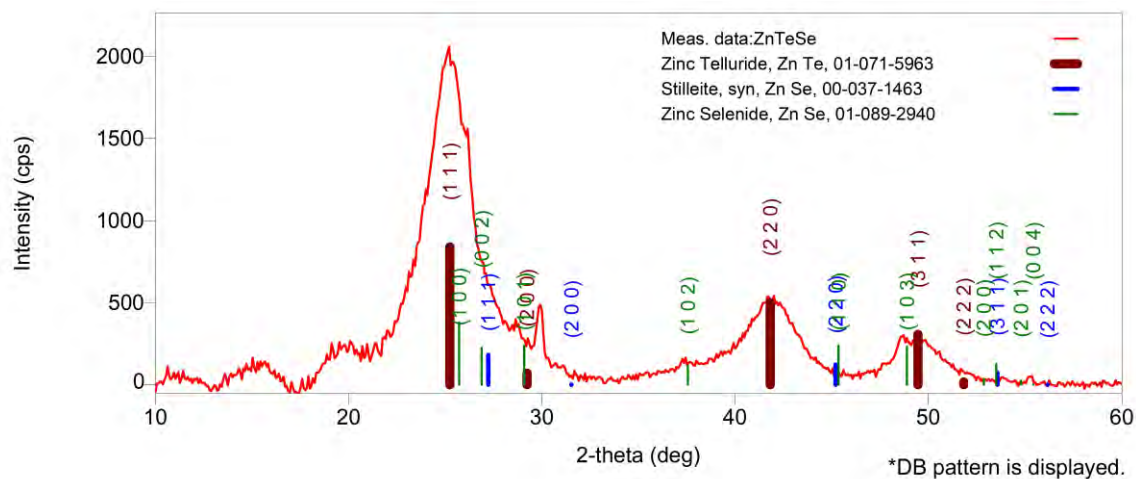
Figure 21: Intensity of X-ray diffraction from ZnTe/ ZnSe QDs.
