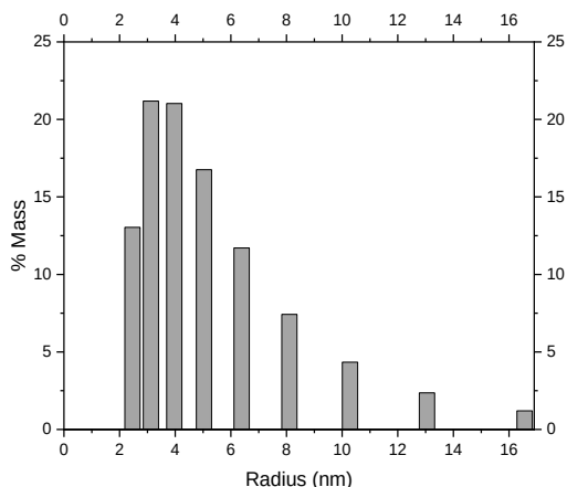
Figure 14: DLS results show the hydrodynamic size distribution of ZnTe/ZnS QDs.
