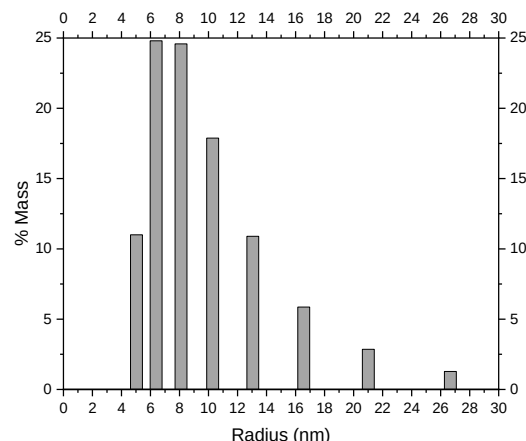
Figure 15: DLS results show the hydrodynamic size distribution of ZnTe/ZnSe QDs.
