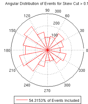
FIGURE 4.10: Angular Distribution for a skew magnitude cut at 0.1.
