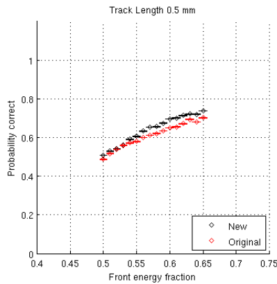
FIGURE 3.11: Fraction Correct as a function of front fractional energy, holding length constant.
