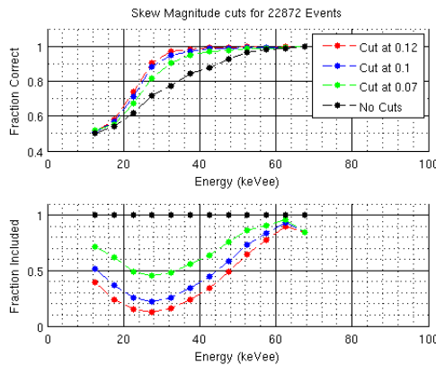
FIGURE 3.23: Top: The fraction of events correct at a given energy with three cuts excluding events below the listed skewness magnitude. Bottom: The fraction of events included at each point in the top plot. (Saxophone Plot)
