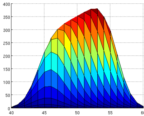
FIGURE 2.7: Image projected into x - z plane.
