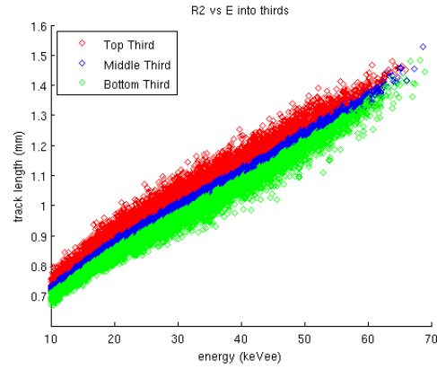
FIGURE 3.22: The same plot, divided into thirds. The blue seems smaller than the red and green because the events are more densely clustered.
