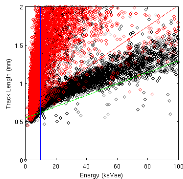
FIGURE 4.3: Red events have a skewness magnitude above 0.9.
