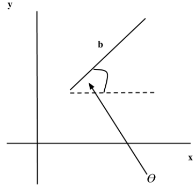
FIGURE A.2: Looking down on the same track in the x-y plane. The track makes an angle \theta with the x-axis.
